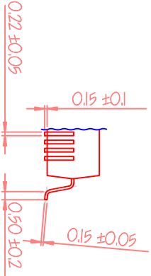
DETAIL B (5=5/1)
