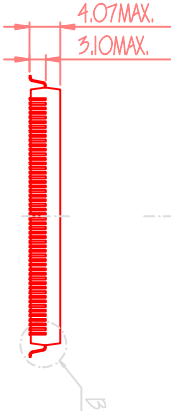
DETAIL B (5=5/1)
