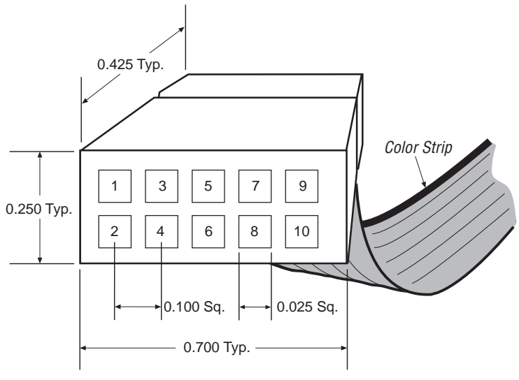
Figure 1. 10-Pin Female Plug Dimensions
