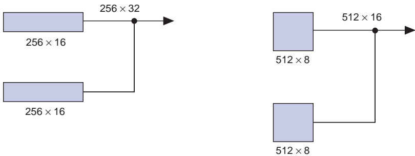
Figure 6. Examples of Combining ACEX 1K EABs
